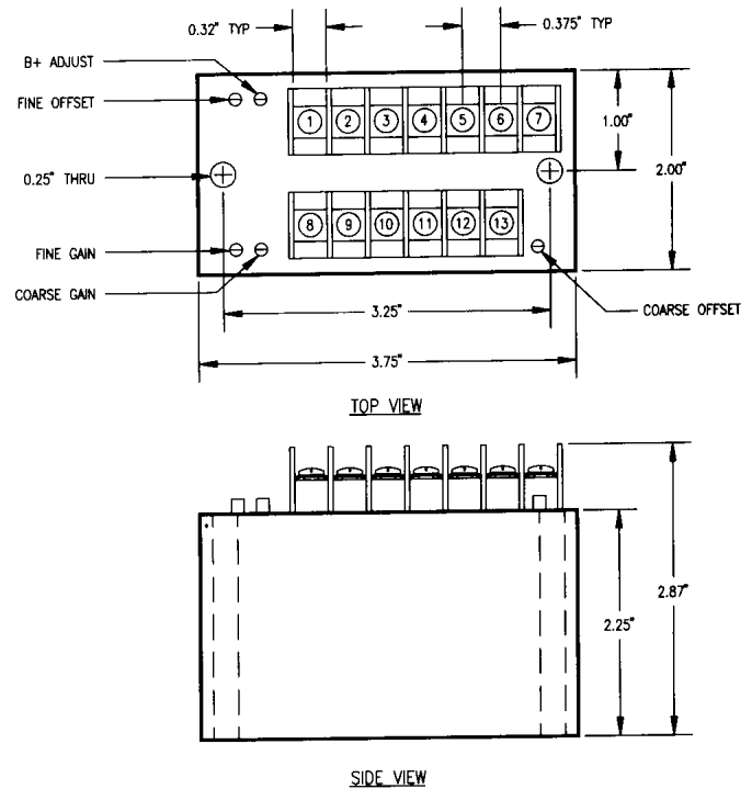
FIGURE 5. Case Dimension
