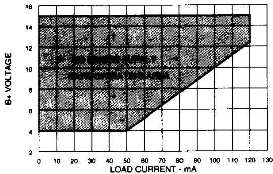
FIGURE 2. Safe Operating Curve
