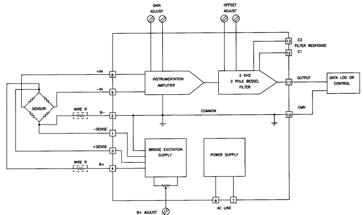
FIGURE 3. Typical Bridge Application
